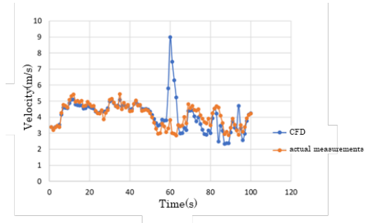
Fig 14 Comparison of rooftop wind velocity
